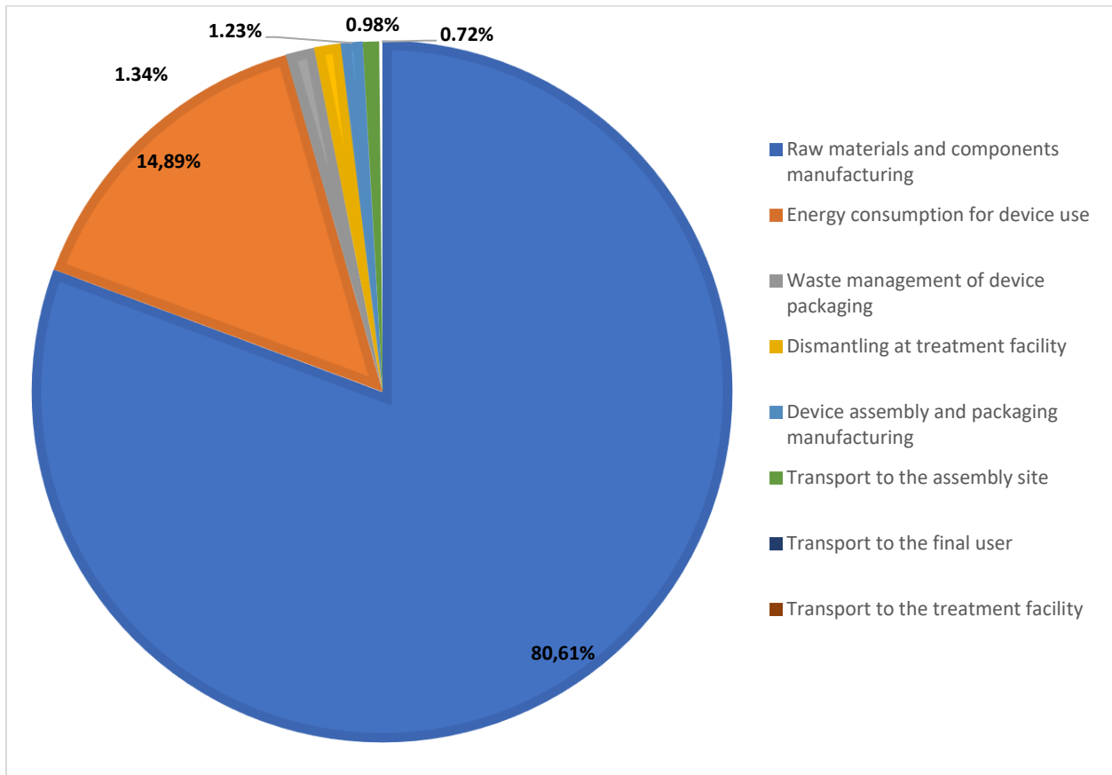
Contribution of each life cycle stage to GWP impacts- Astro Horizon T11750
