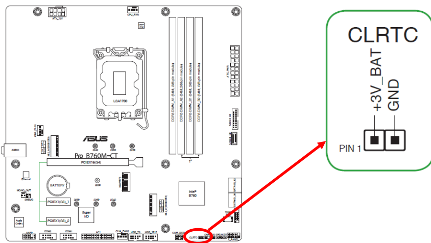
Location of the BIOS Configuration Jumper Block
