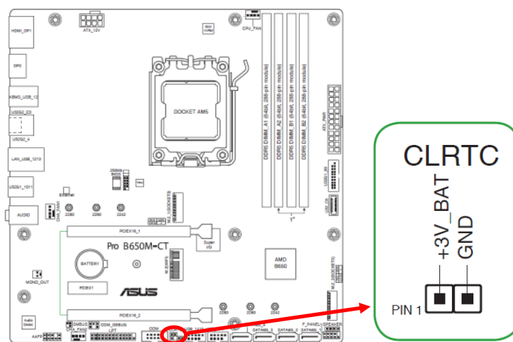
Location of the BIOS Configuration Jumper Block
