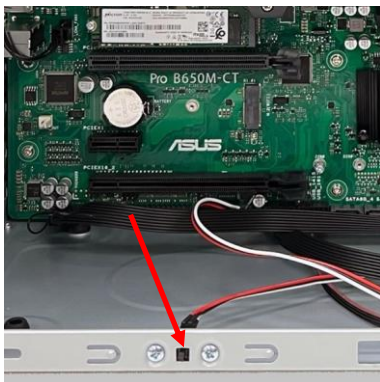
Intrusion switch
