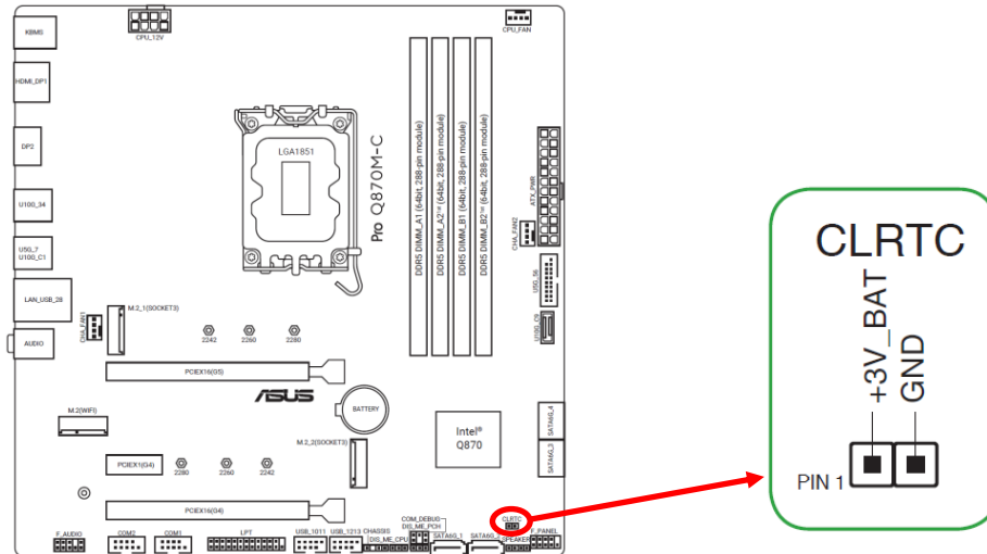
Location of the BIOS Configuration Jumper Block
