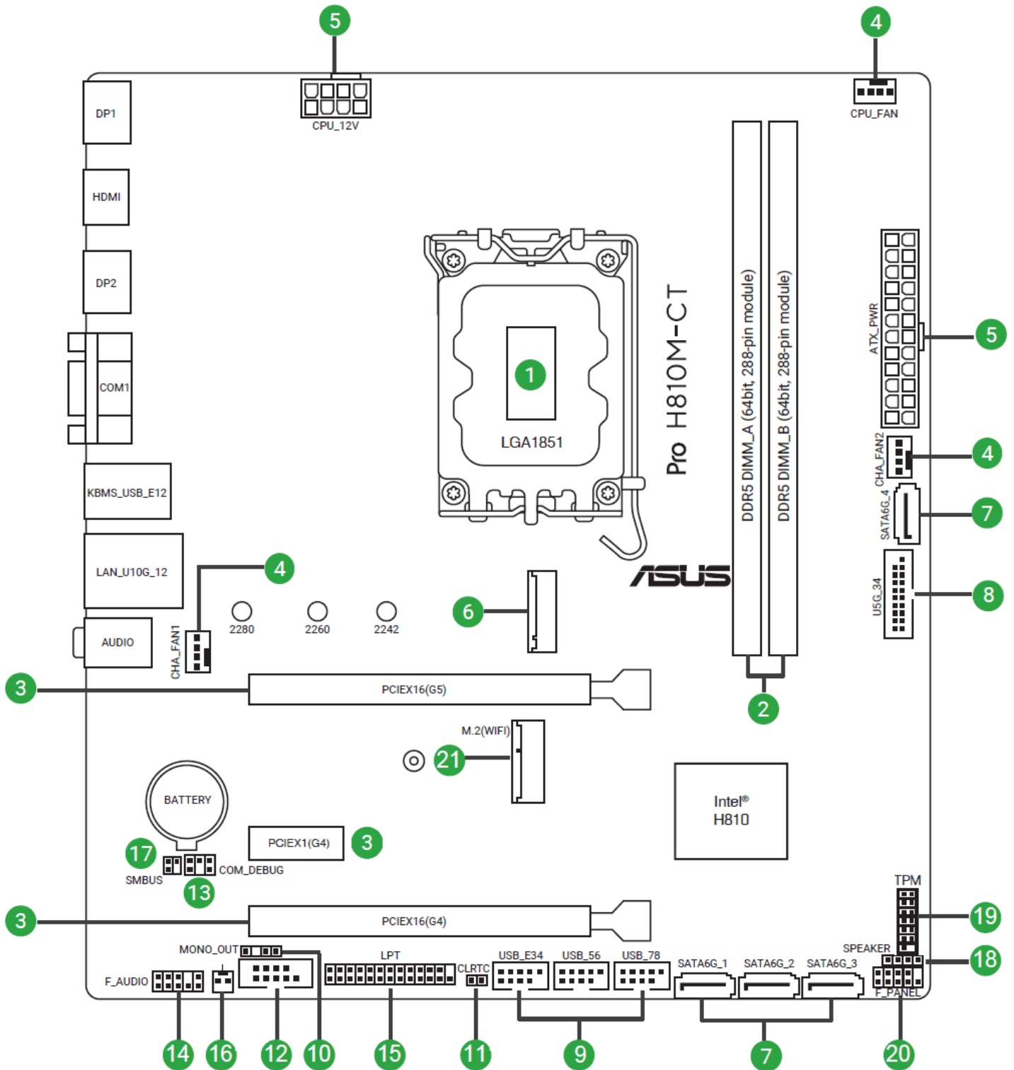
Figure 4.4 Major board components
