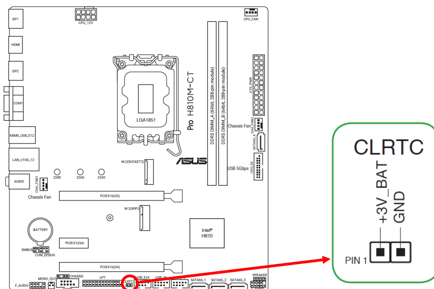
Location of the BIOS Configuration Jumper Block
