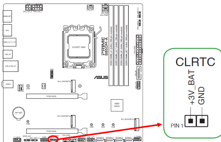
Location of the BIOS Configuration Jumper Block
